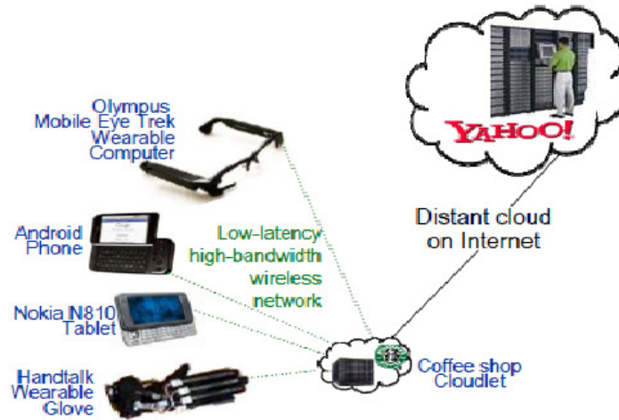
Figure 4. Cloudlet Customization
