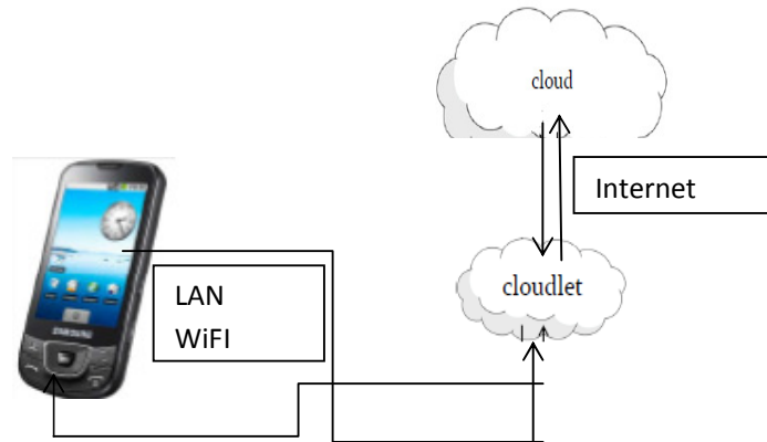
Figure 1. Cloudlets
