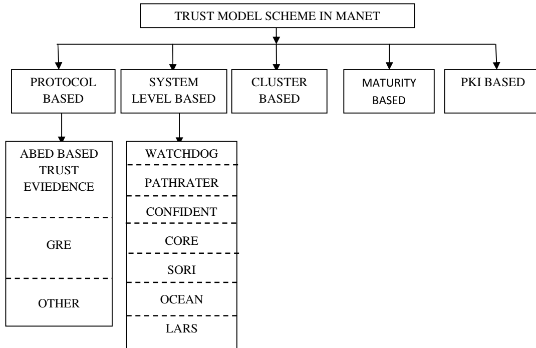
Figure 1. Trust Based Schemes in MANET
