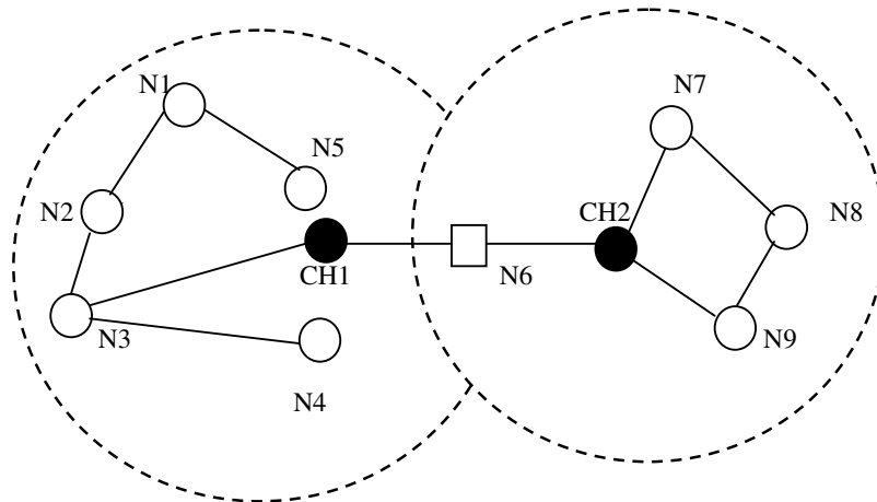
Figure 2. Cluster Based Trust Model in MANET
