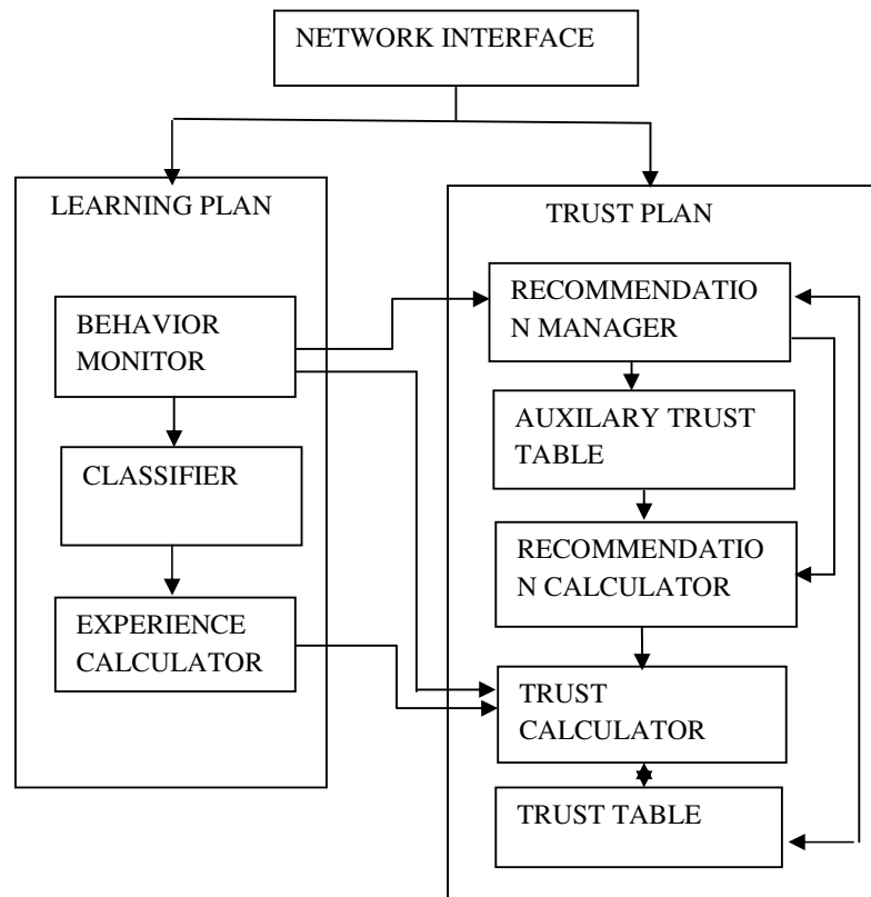
Figure 5. Maturity Based Trust Model
