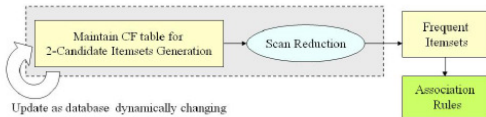
Figure 4: The concept of SWF algorithm for mining association rule
