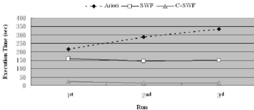
Figure 11: Experimental results when handling log data with dynamically sliding window change
