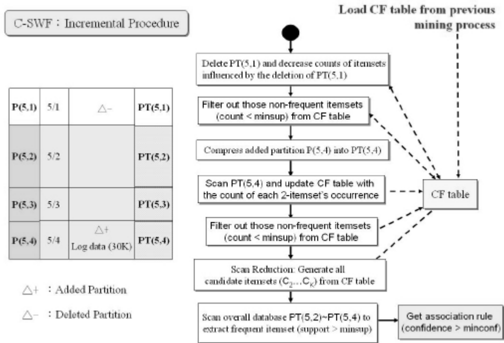
Figure 7: C-SWF algorithm: flow diagram of incremental procedure
