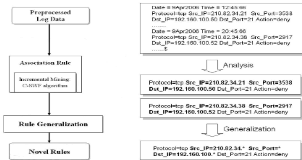
Figure 2: Rule analysis procedure for firewall policy rules generalization
