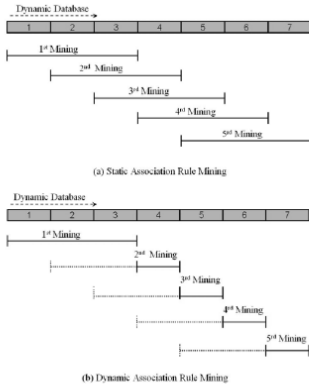
Figure 3: The difference between static and dynamic mining
