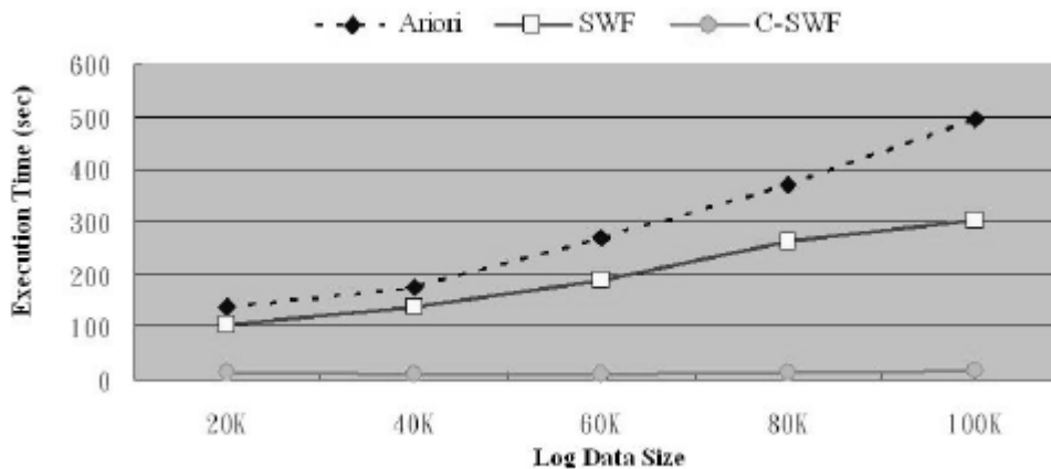
Figure 10: Experimental results when handling incremental log data
