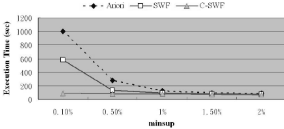
Figure 9: Experimental results when handling large amount of log data
