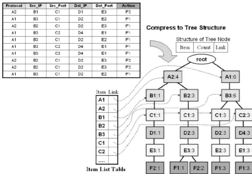
Figure 5: The structure of compression log tree
