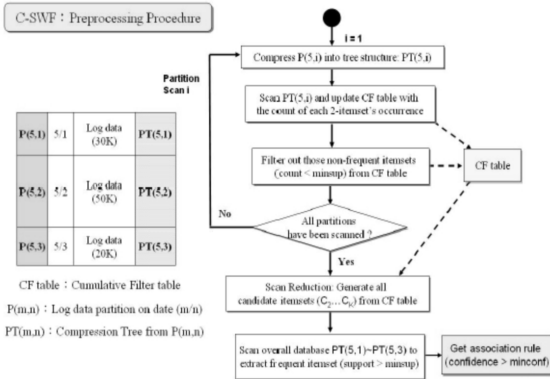
Figure 6: C-SWF algorithm: flow diagram of preprocessing procedure
