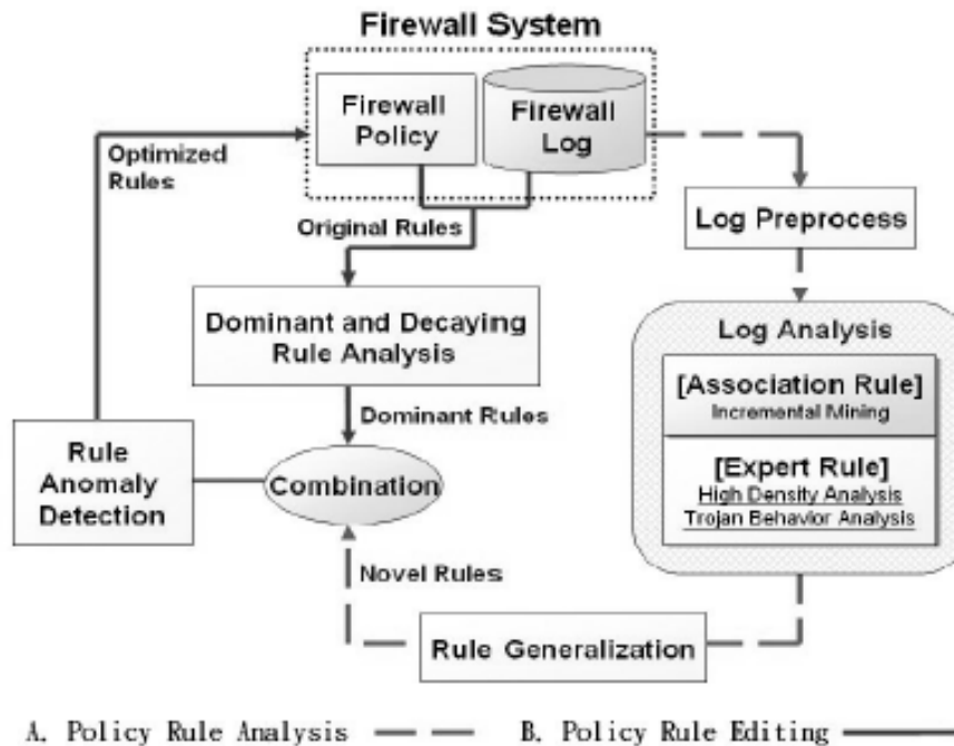
Figure 1: Proposed firewall policy management system architecture
