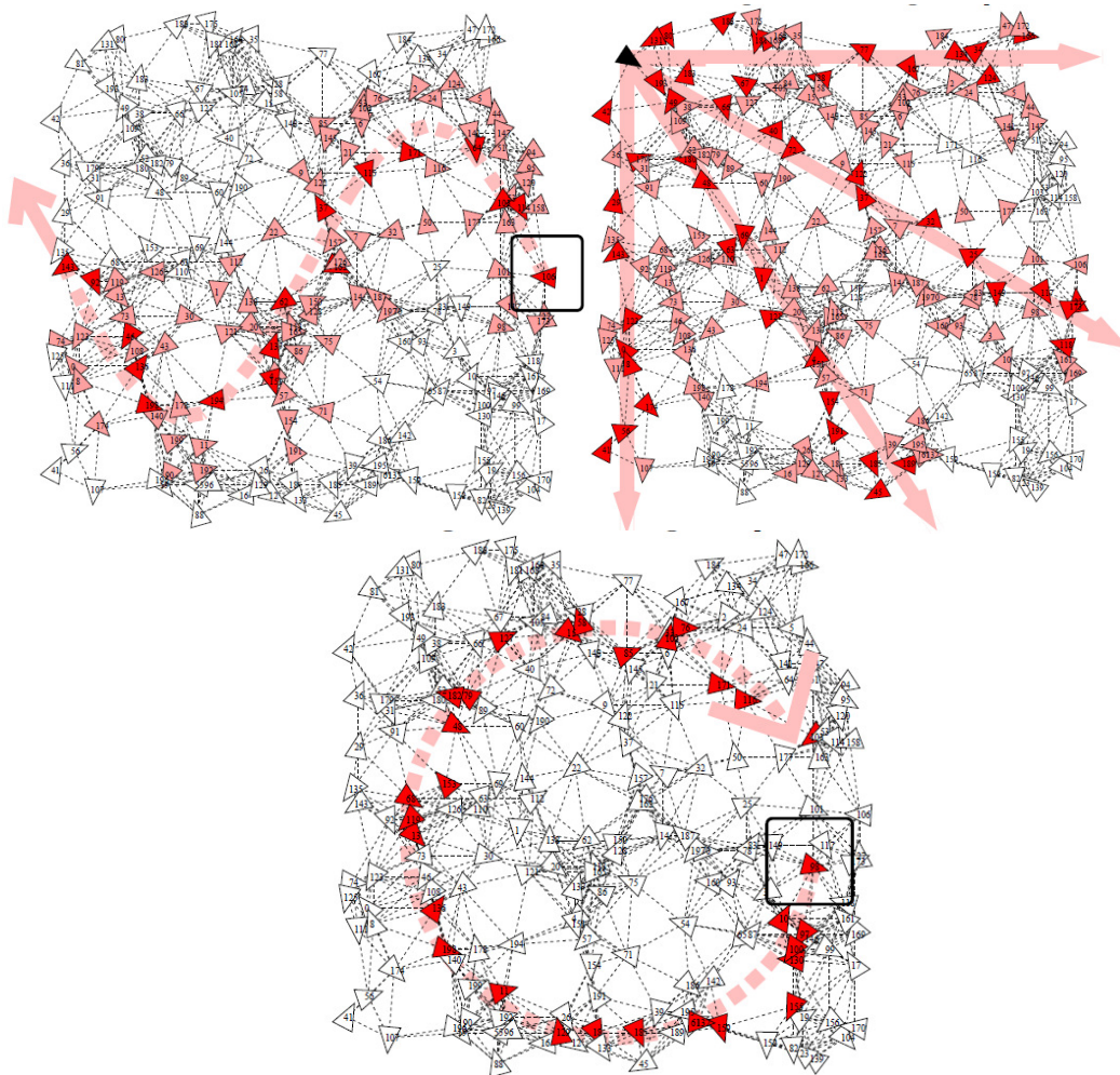
Figure 10. TBF architecture
