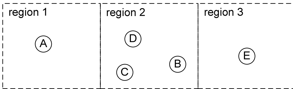
Figure 8. GAF architecture
