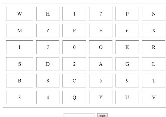
Figure 7: Login interface
