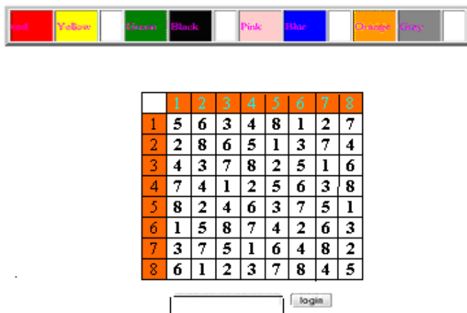
Figure 10: Login interface
