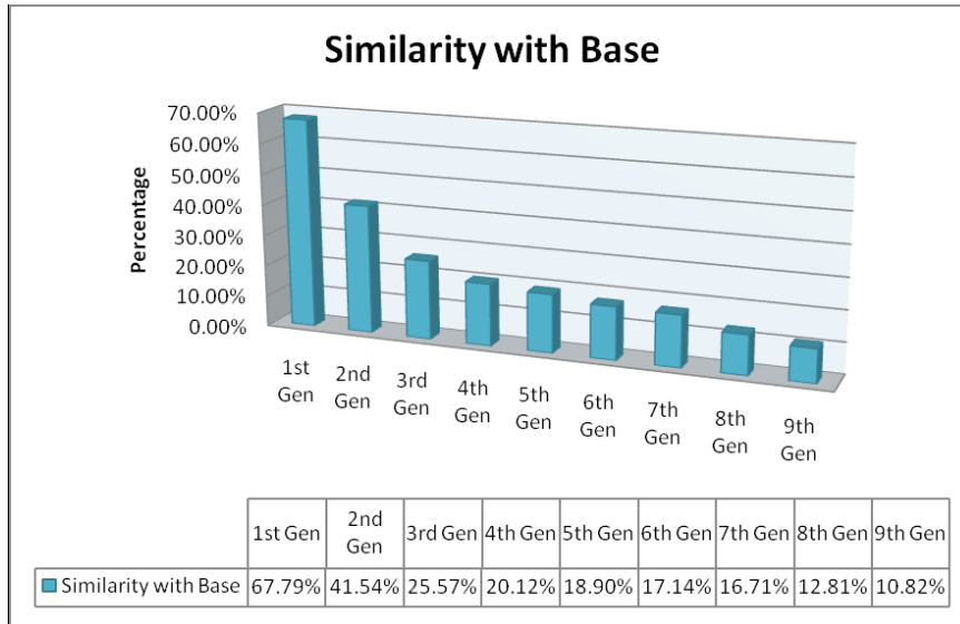
Figure 9: Similarity results of the base virus v/s 9 different generations
