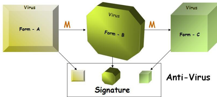
Figure 1: Metamorphic virus generations
