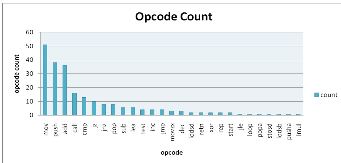
Figure 6: Base virus opcodes and their frequency
