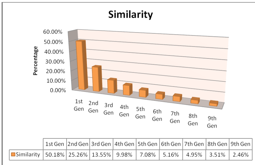
Figure 10: Graph of Similarity of two N generations
