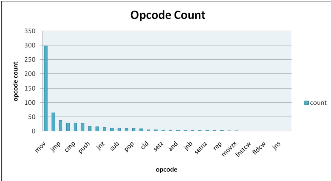
Figure 7: Opcodes of normal file and their frequency
