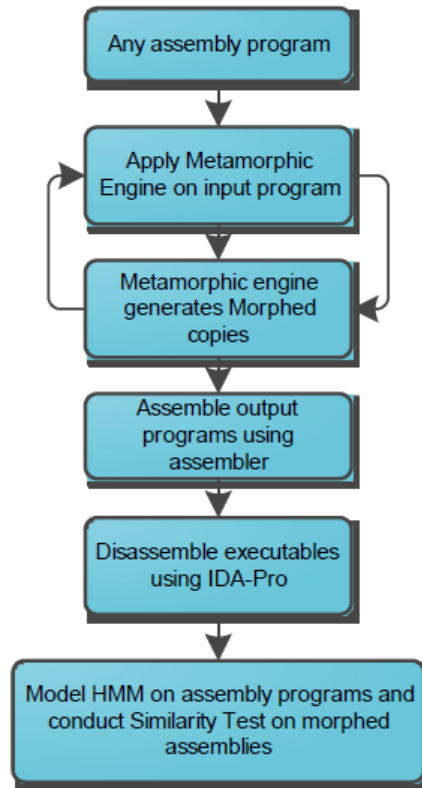
Figure 8: All over Process
